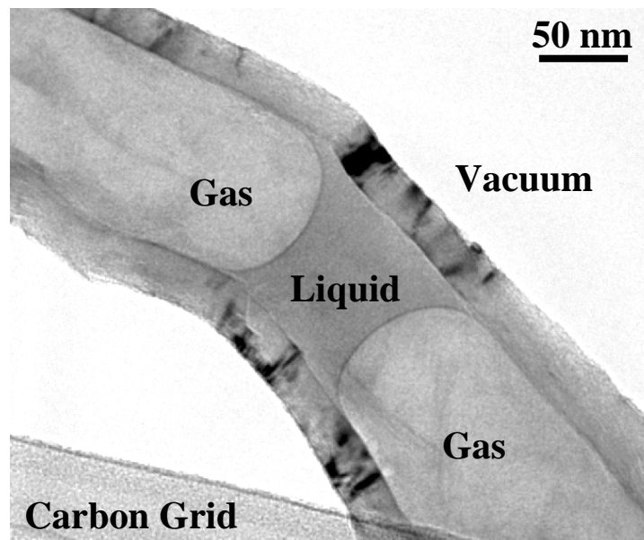
Fig. 2. TEM image of the elbow portion of a carbon nanotube. This tube is capped at both ends and contains a liquid inclusion constrained between two curved menisci separating the aqueous liquid from the adjoining gas. The nanotube rests on a holey carbon grid, a segment of which is visible in the lower left corner of the micrograph. The environment outside the nanotube is the high vacuum of the TEM column. The volume of the liquid inclusion is of the order of 10^{-18} ( atto ) liters. The contact angles varied between 0 and 25 degrees.
