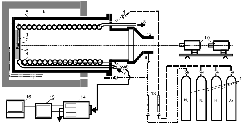
Fig.1. Scheme of the measurement stand; 1- sample of steel, 2-bottom plate, 3-thermocouples, 4-water jacket, 5-measurement capsule, 6-furnace chamber, 7,8-water outlet/inlet, 9-inlet/outlet of protection gas, 10-pyrometers, 11-protection gases, 12-eyehole, 13-rotameters, 14-gas analysers, 15-data logger, 16-computer
